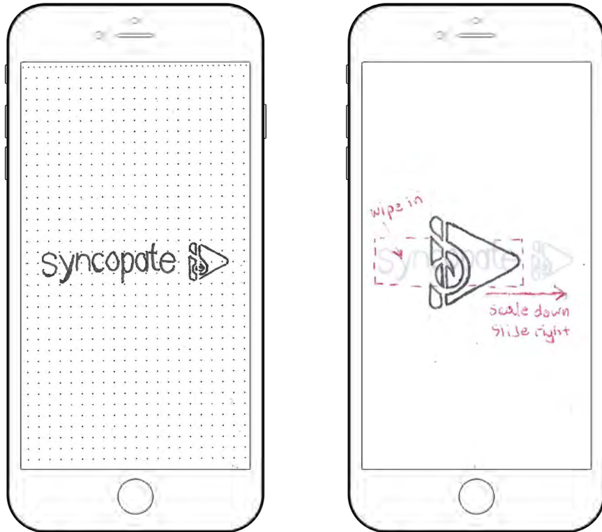
Opening Screen
