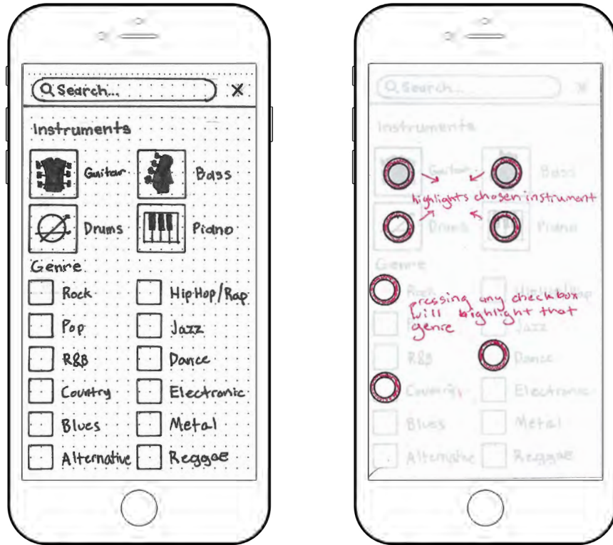
Search Screen
