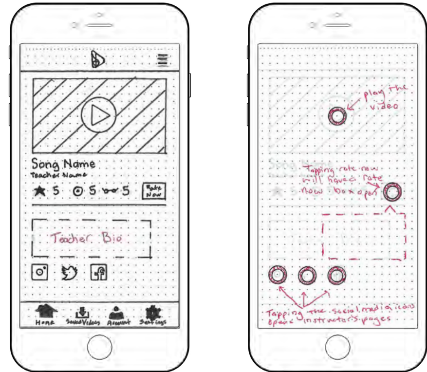
Video Screen
