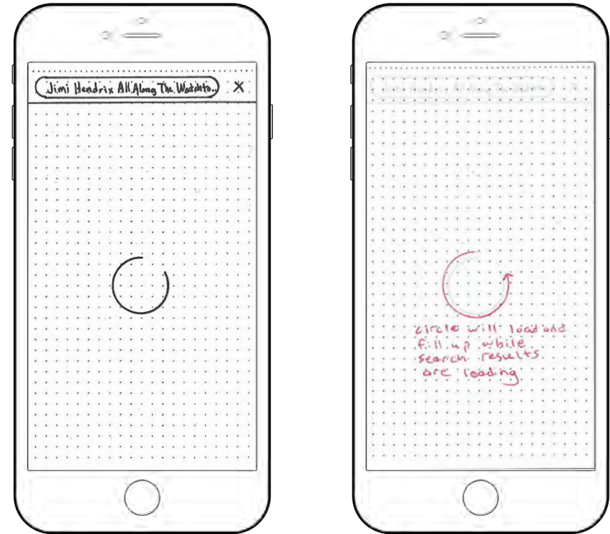
Loading Screen
