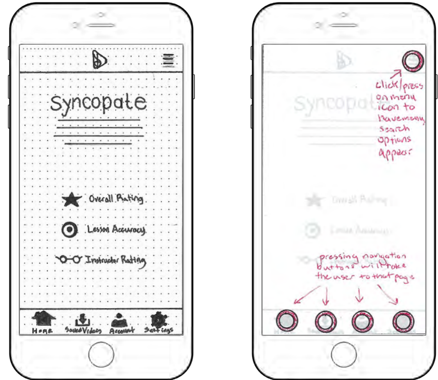
Home Screen
